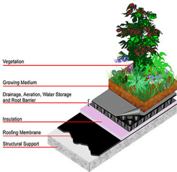
Exhibit B: Green Roof Schematic Courtesy of American Wick
